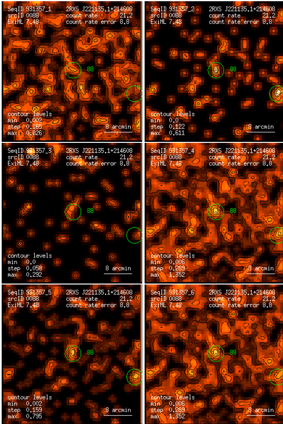
Figure 88: RASS 931357: detection 0088: band rate images, Gaussian filter: (1) PSPC channels 11 – 41, (2) 52 – 90, (3) 91 – 201, (4) 11 – 235, (5) 52 – 201, (6) 11 – 201. Broad band rates in counts/ks. Band rate contour levels in counts/ks/arcmin 2 .
