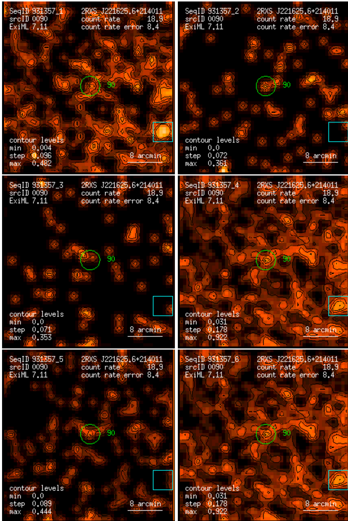
Figure 90: RASS 931357: detection 0090: band rate images, Gaussian filter: (1) PSPC channels 11 – 41, (2) 52 – 90, (3) 91 – 201, (4) 11 – 235, (5) 52 – 201, (6) 11 – 201. Broad band rates in counts/ks. Band rate contour levels in counts/ks/arcmin 2 .
