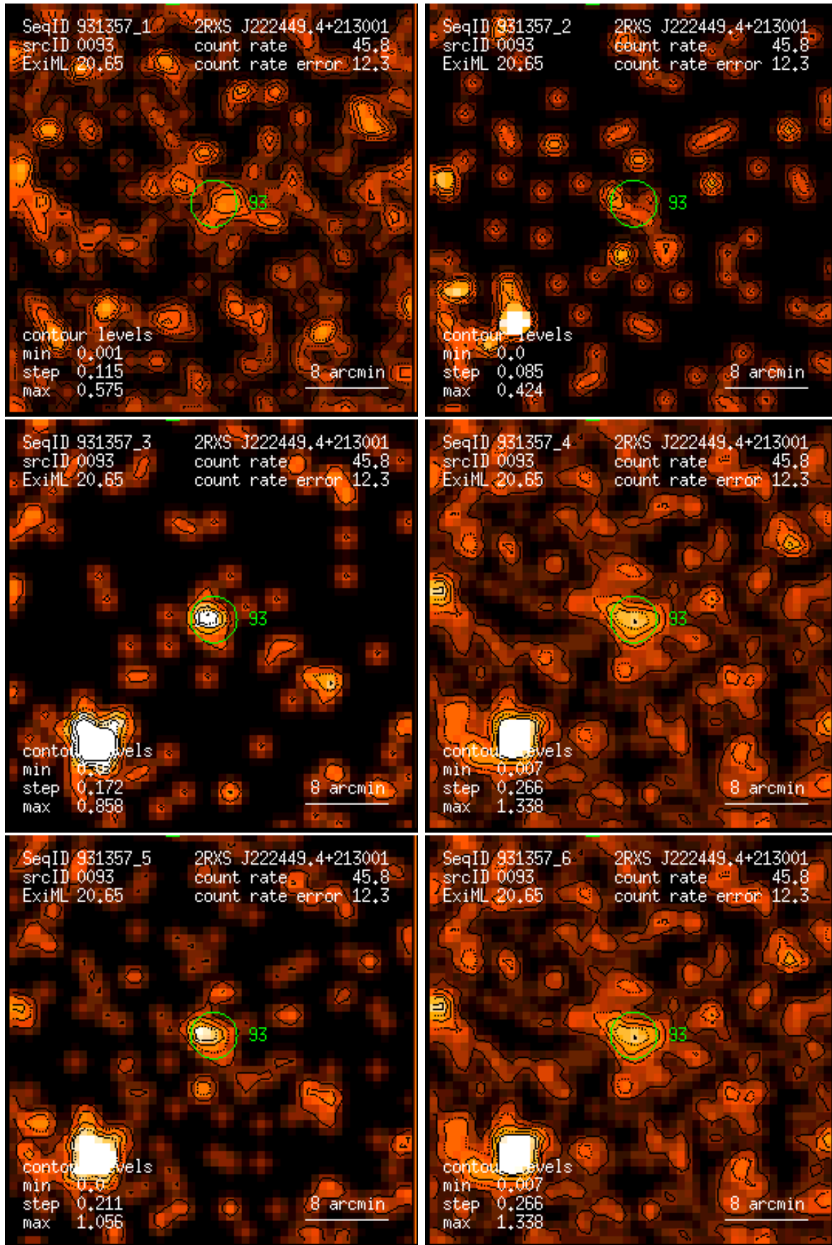
Figure 93: RASS 931357: detection 0093: band rate images, Gaussian filter: (1) PSPC channels 11 – 41, (2) 52 – 90, (3) 91 – 201, (4) 11 – 235, (5) 52 – 201, (6) 11 – 201. Broad band rates in counts/ks. Band rate contour levels in counts/ks/arcmin 2 .
