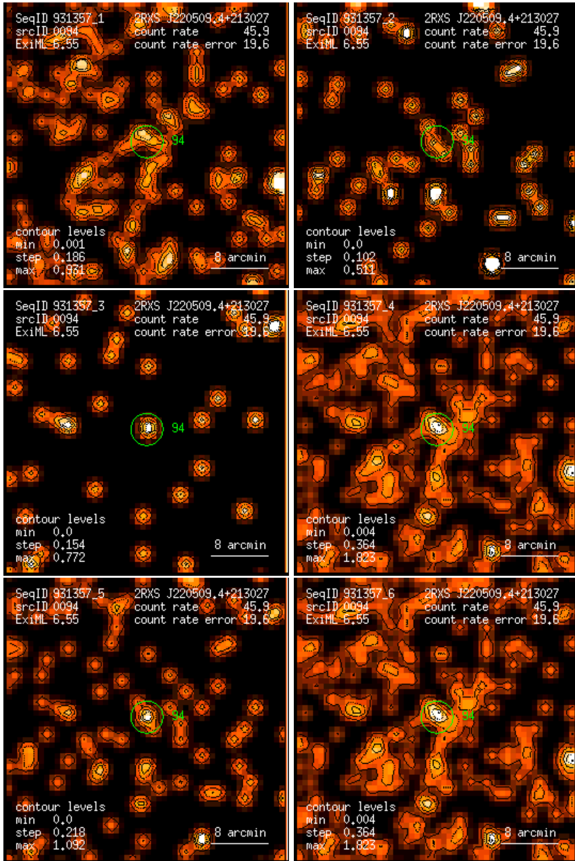
Figure 94: RASS 931357: detection 0094: band rate images, Gaussian filter: (1) PSPC channels 11 – 41, (2) 52 – 90, (3) 91 – 201, (4) 11 – 235, (5) 52 – 201, (6) 11 – 201. Broad band rates in counts/ks. Band rate contour levels in counts/ks/arcmin 2 .
