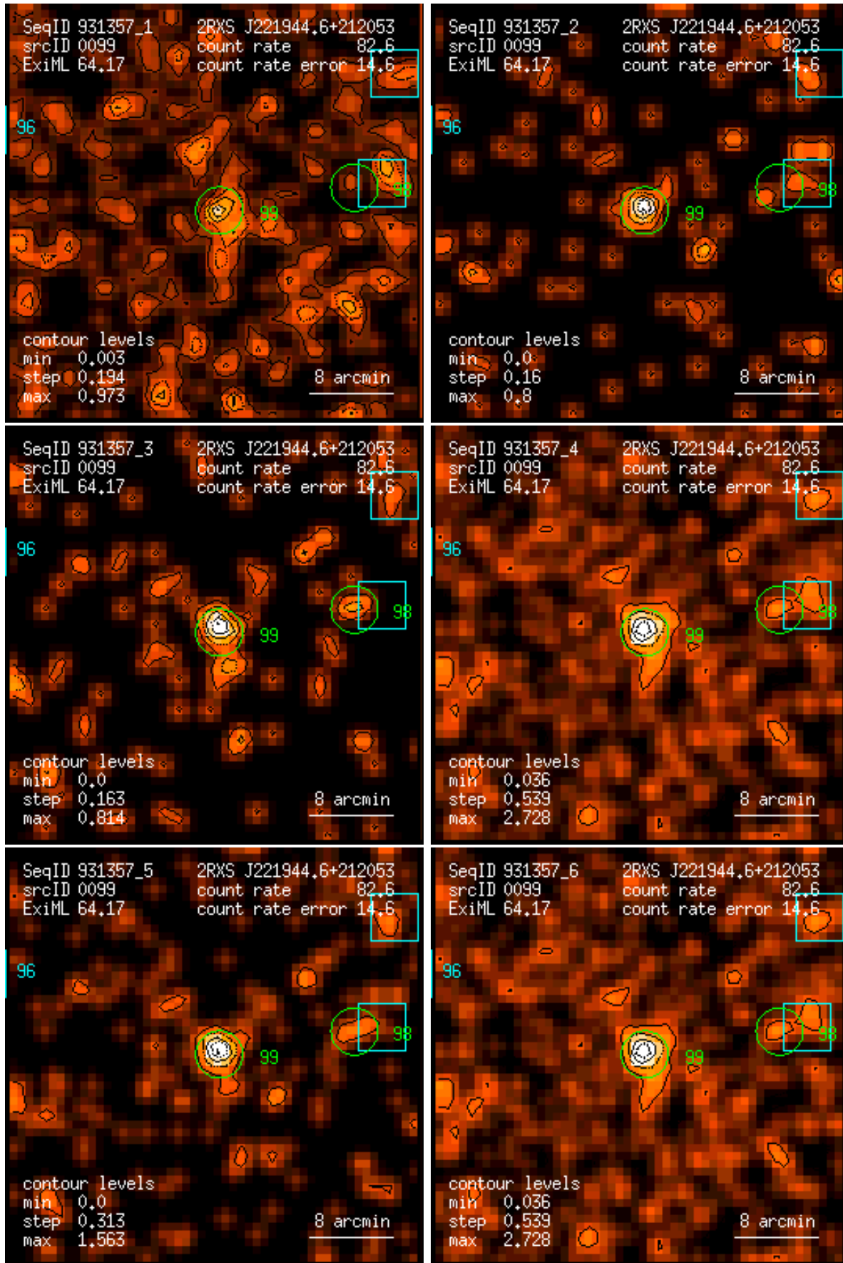
Figure 99: RASS 931357: detection 0099: band rate images, Gaussian filter: (1) PSPC channels 11 – 41, (2) 52 – 90, (3) 91 – 201, (4) 11 – 235, (5) 52 – 201, (6) 11 – 201. Broad band rates in counts/ks. Band rate contour levels in counts/ks/arcmin 2 .
