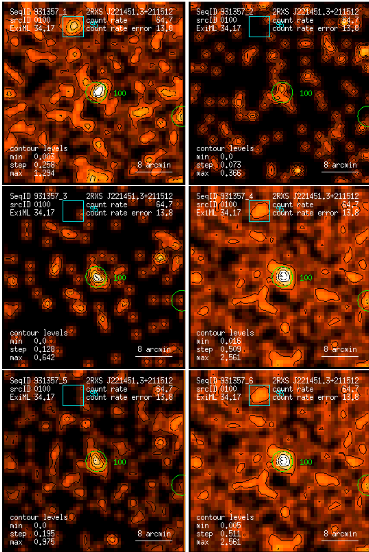
Figure 100: RASS 931357: detection 0100: band rate images, Gaussian filter: (1) PSPC channels 11 – 41, (2) 52 – 90, (3) 91 – 201, (4) 11 – 235, (5) 52 – 201, (6) 11 – 201. Broad band rates in counts/ks. Band rate contour levels in counts/ks/arcmin 2 .
