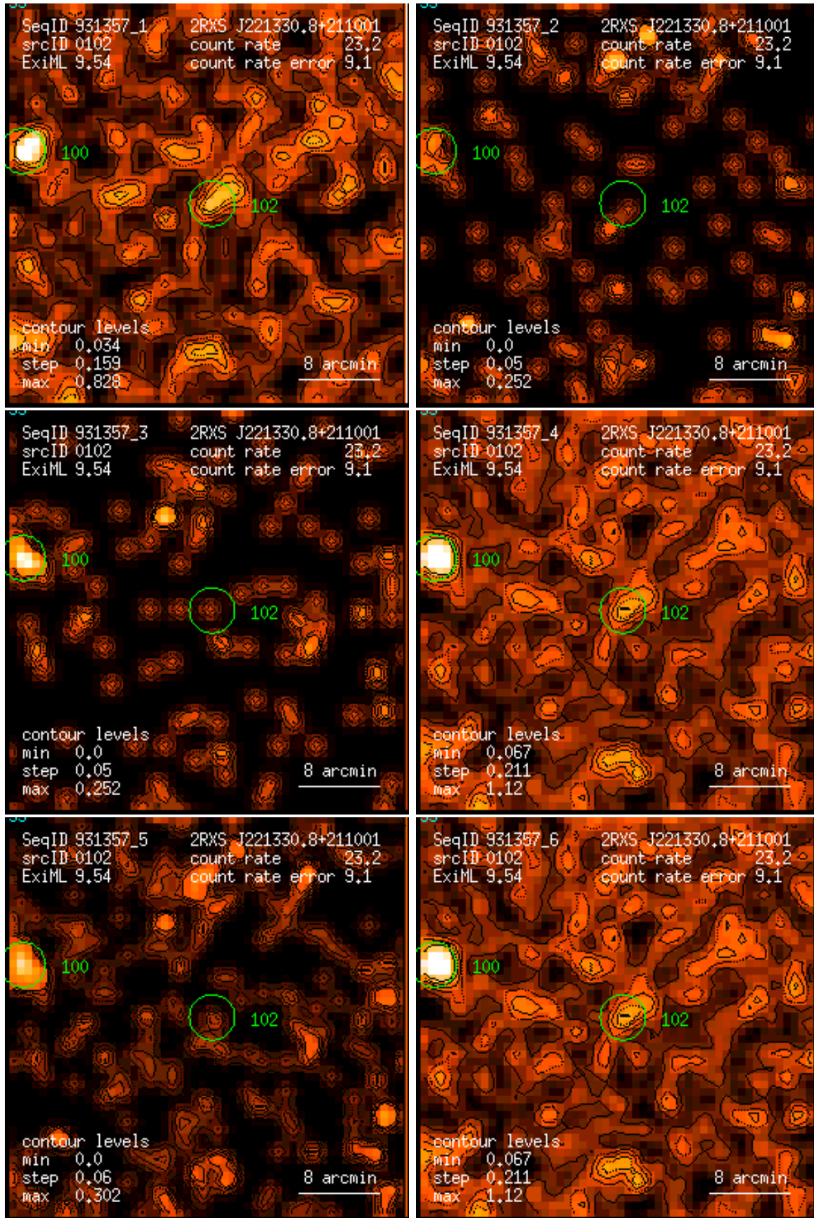
Figure 102: RASS 931357: detection 0102: band rate images, Gaussian filter: (1) PSPC channels 11 – 41, (2) 52 – 90, (3) 91 – 201, (4) 11 – 235, (5) 52 – 201, (6) 11 – 201. Broad band rates in counts/ks. Band rate contour levels in counts/ks/arcmin 2 .
