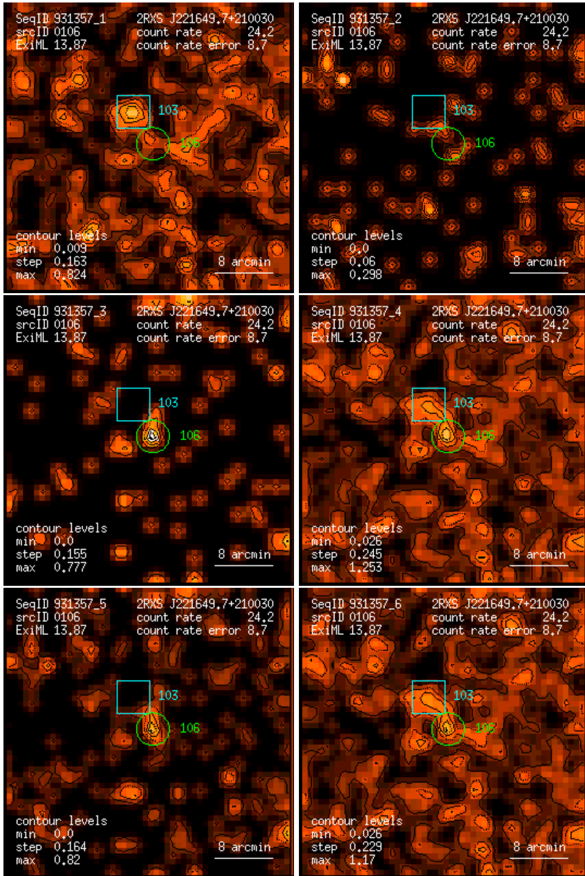
Figure 106: RASS 931357: detection 0106: band rate images, Gaussian filter: (1) PSPC channels 11 – 41, (2) 52 – 90, (3) 91 – 201, (4) 11 – 235, (5) 52 – 201, (6) 11 – 201. Broad band rates in counts/ks. Band rate contour levels in counts/ks/arcmin 2 .
