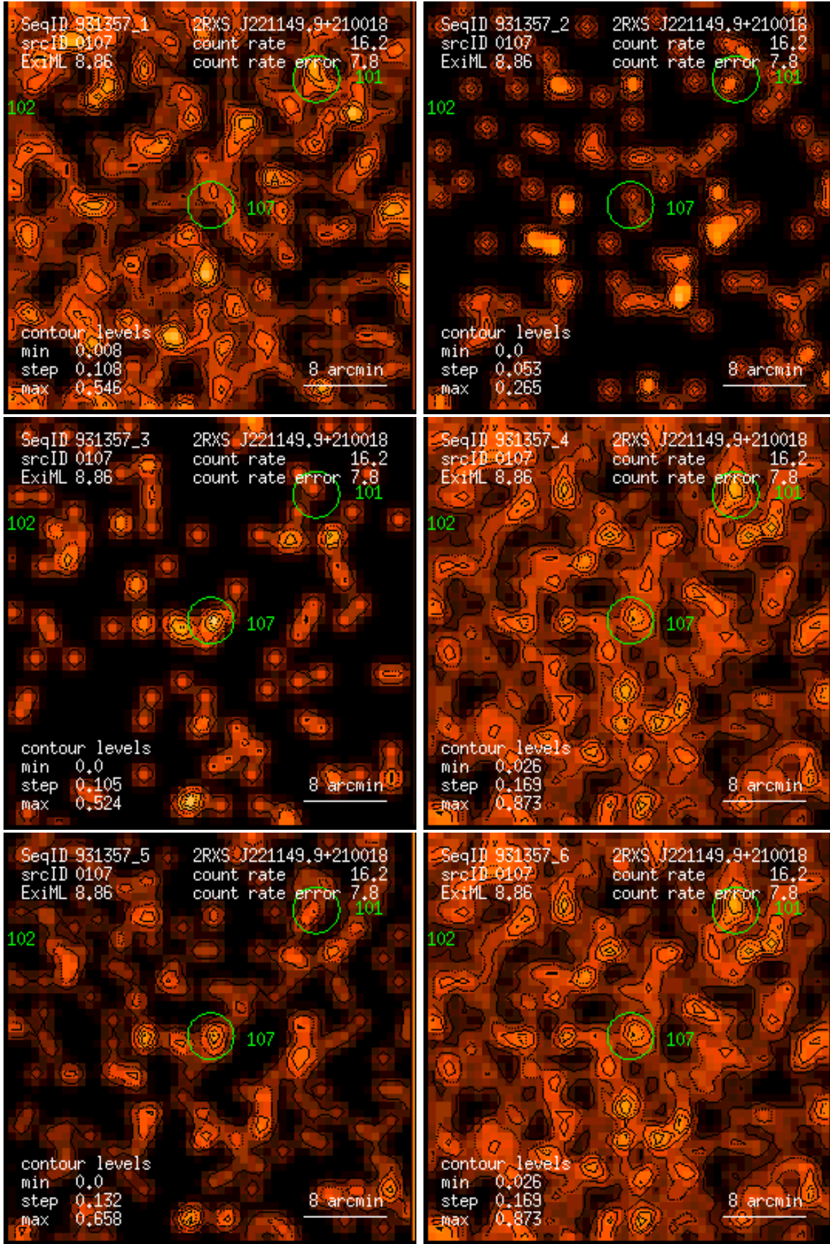
Figure 107: RASS 931357: detection 0107: band rate images, Gaussian filter: (1) PSPC channels 11 – 41, (2) 52 – 90, (3) 91 – 201, (4) 11 – 235, (5) 52 – 201, (6) 11 – 201. Broad band rates in counts/ks. Band rate contour levels in counts/ks/arcmin 2 .
