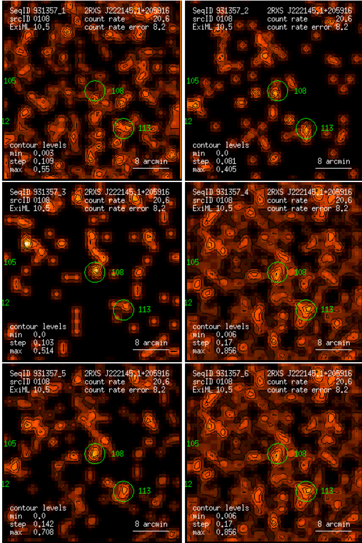
Figure 108: RASS 931357: detection 0108: band rate images, Gaussian filter: (1) PSPC channels 11 – 41, (2) 52 – 90, (3) 91 – 201, (4) 11 – 235, (5) 52 – 201, (6) 11 – 201. Broad band rates in counts/ks. Band rate contour levels in counts/ks/arcmin 2 .
