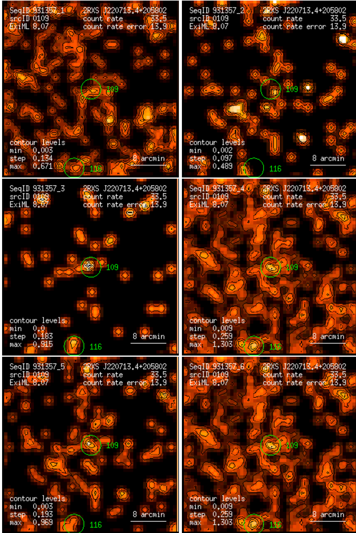
Figure 109: RASS 931357: detection 0109: band rate images, Gaussian filter: (1) PSPC channels 11 – 41, (2) 52 – 90, (3) 91 – 201, (4) 11 – 235, (5) 52 – 201, (6) 11 – 201. Broad band rates in counts/ks. Band rate contour levels in counts/ks/arcmin 2 .
