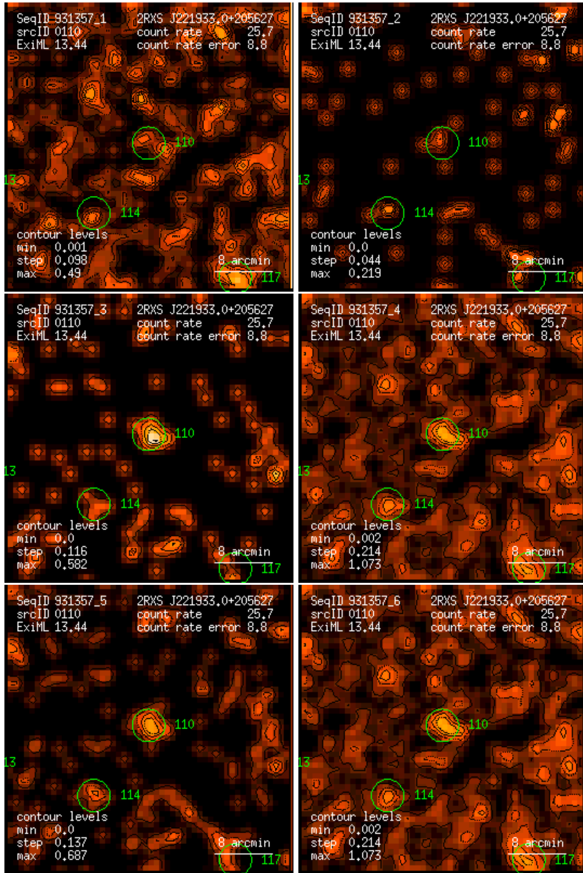
Figure 110: RASS 931357: detection 0110: band rate images, Gaussian filter: (1) PSPC channels 11 – 41, (2) 52 – 90, (3) 91 – 201, (4) 11 – 235, (5) 52 – 201, (6) 11 – 201. Broad band rates in counts/ks. Band rate contour levels in counts/ks/arcmin 2 .
