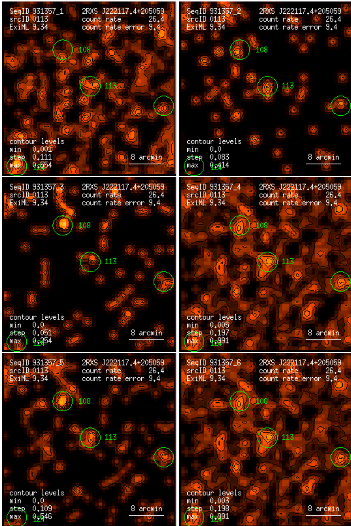
Figure 113: RASS 931357: detection 0113: band rate images, Gaussian filter: (1) PSPC channels 11 – 41, (2) 52 – 90, (3) 91 – 201, (4) 11 – 235, (5) 52 – 201, (6) 11 – 201. Broad band rates in counts/ks. Band rate contour levels in counts/ks/arcmin 2 .
