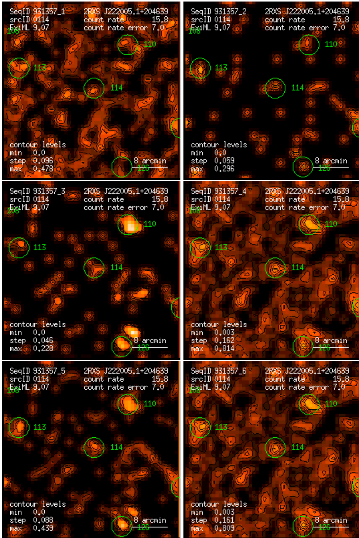
Figure 114: RASS 931357: detection 0114: band rate images, Gaussian filter: (1) PSPC channels 11 – 41, (2) 52 – 90, (3) 91 – 201, (4) 11 – 235, (5) 52 – 201, (6) 11 – 201. Broad band rates in counts/ks. Band rate contour levels in counts/ks/arcmin 2 .
