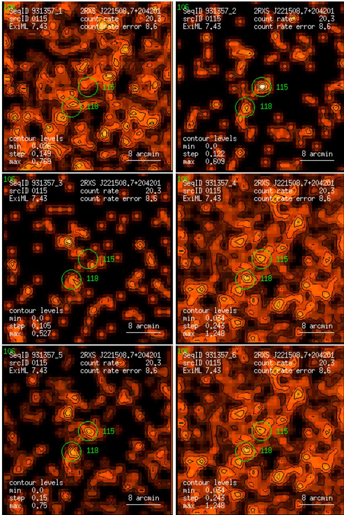
Figure 115: RASS 931357: detection 0115: band rate images, Gaussian filter: (1) PSPC channels 11 – 41, (2) 52 – 90, (3) 91 – 201, (4) 11 – 235, (5) 52 – 201, (6) 11 – 201. Broad band rates in counts/ks. Band rate contour levels in counts/ks/arcmin 2 .
