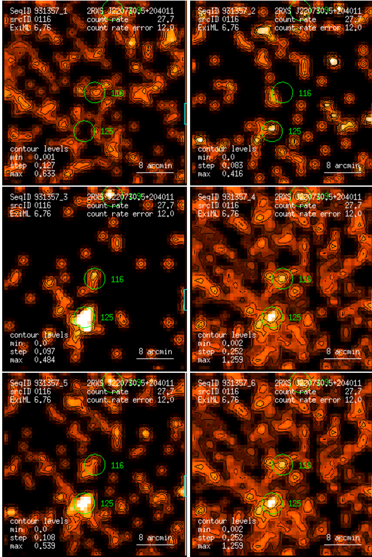
Figure 116: RASS 931357: detection 0116: band rate images, Gaussian filter: (1) PSPC channels 11 – 41, (2) 52 – 90, (3) 91 – 201, (4) 11 – 235, (5) 52 – 201, (6) 11 – 201. Broad band rates in counts/ks. Band rate contour levels in counts/ks/arcmin 2 .
