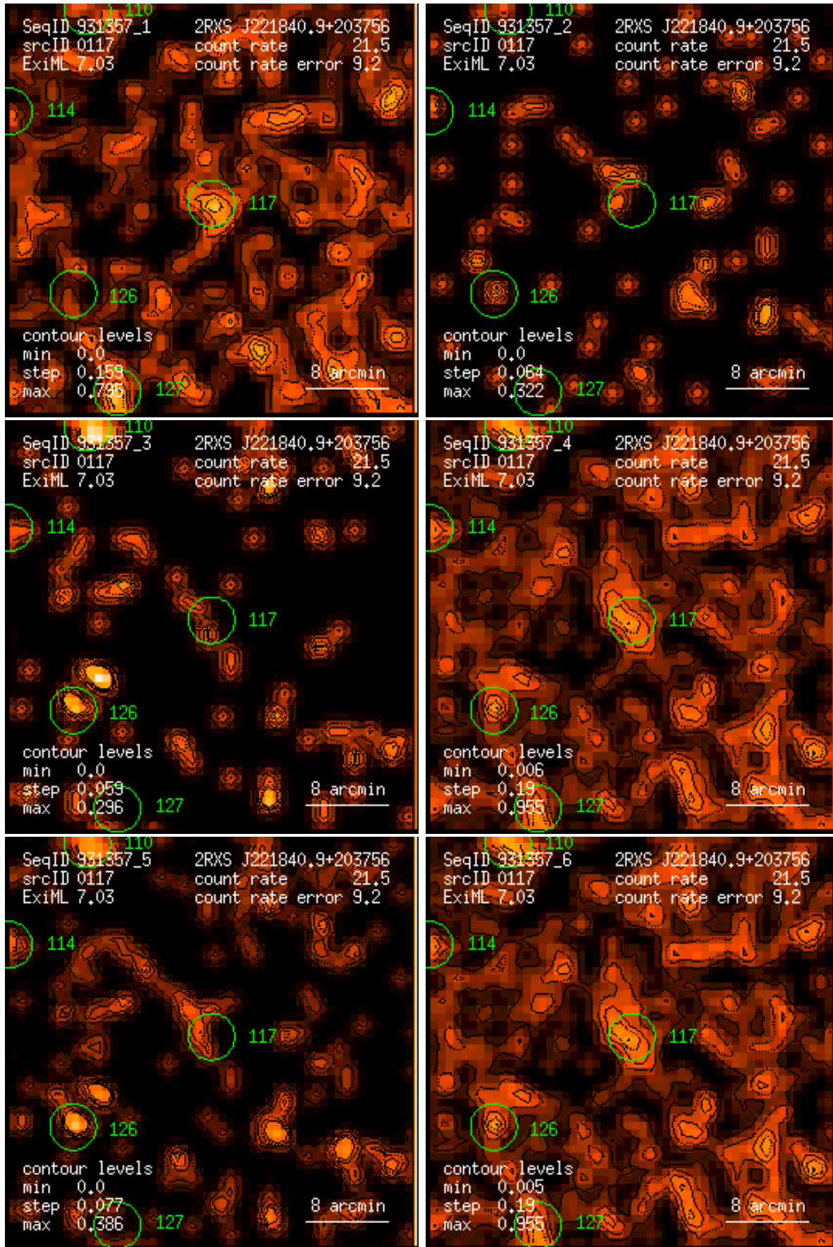
Figure 117: RASS 931357: detection 0117: band rate images, Gaussian filter: (1) PSPC channels 11 – 41, (2) 52 – 90, (3) 91 – 201, (4) 11 – 235, (5) 52 – 201, (6) 11 – 201. Broad band rates in counts/ks. Band rate contour levels in counts/ks/arcmin 2 .
