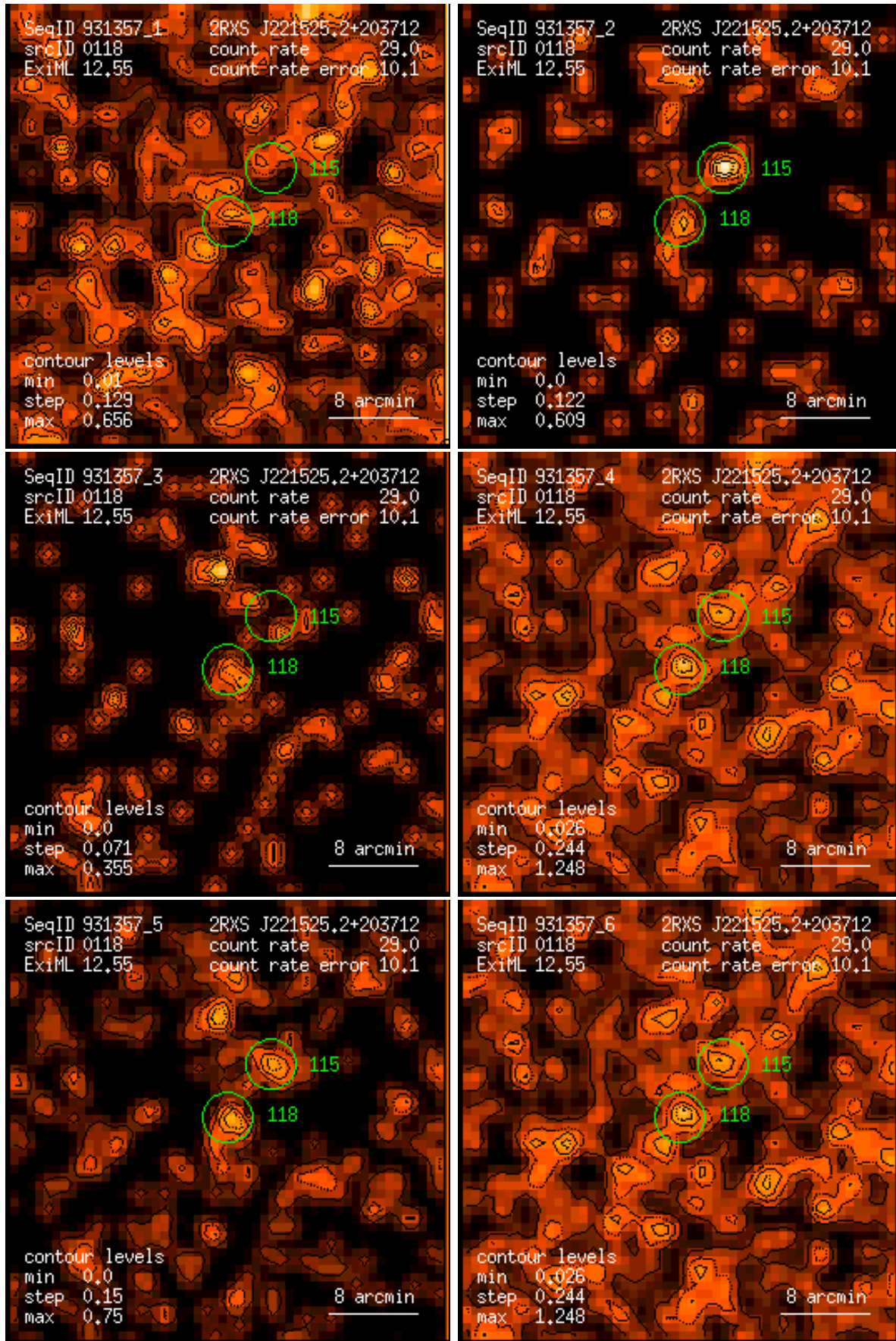
Figure 118: RASS 931357: detection 0118: band rate images, Gaussian filter: (1) PSPC channels 11 – 41, (2) 52 – 90, (3) 91 – 201, (4) 11 – 235, (5) 52 – 201, (6) 11 – 201. Broad band rates in counts/ks. Band rate contour levels in counts/ks/arcmin 2 .
