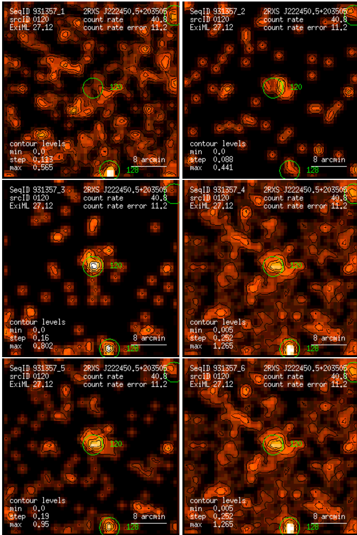
Figure 120: RASS 931357: detection 0120: band rate images, Gaussian filter: (1) PSPC channels 11 – 41, (2) 52 – 90, (3) 91 – 201, (4) 11 – 235, (5) 52 – 201, (6) 11 – 201. Broad band rates in counts/ks. Band rate contour levels in counts/ks/arcmin 2 .
