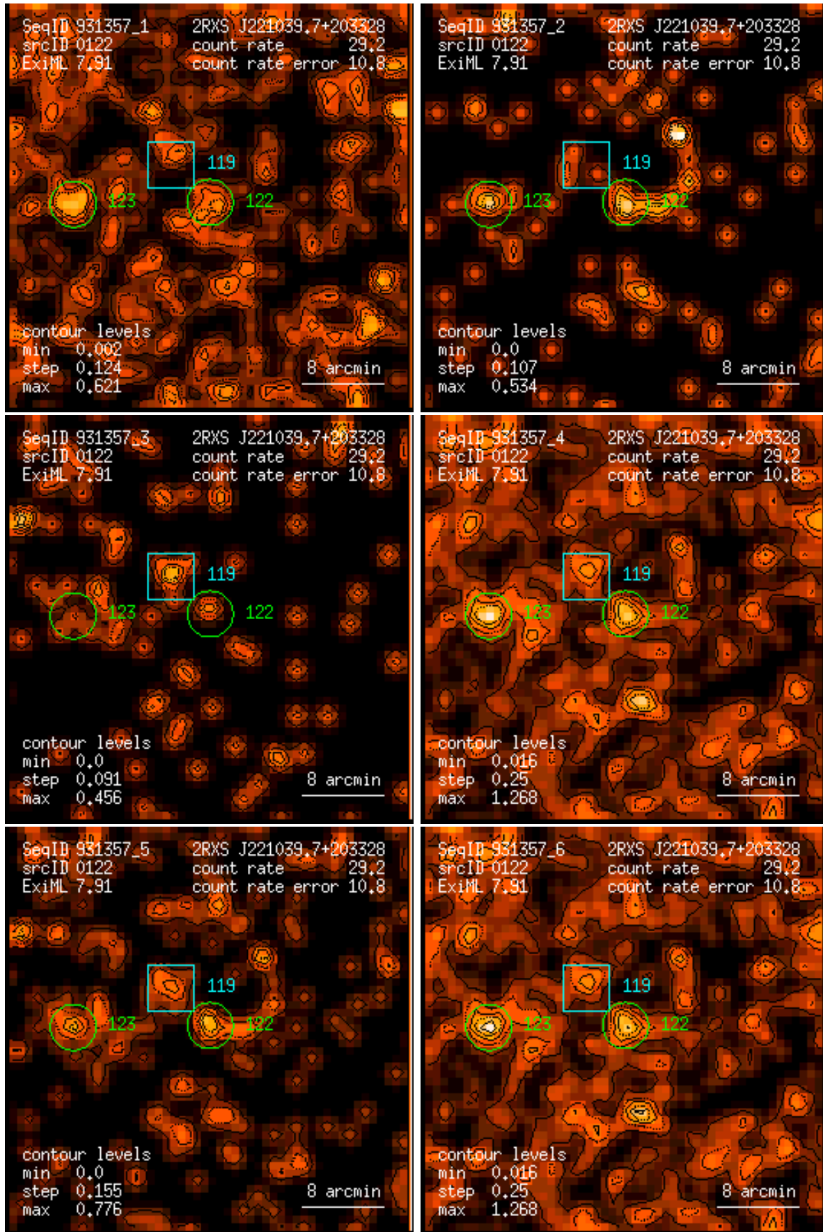
Figure 122: RASS 931357: detection 0122: band rate images, Gaussian filter: (1) PSPC channels 11 – 41, (2) 52 – 90, (3) 91 – 201, (4) 11 – 235, (5) 52 – 201, (6) 11 – 201. Broad band rates in counts/ks. Band rate contour levels in counts/ks/arcmin 2 .
