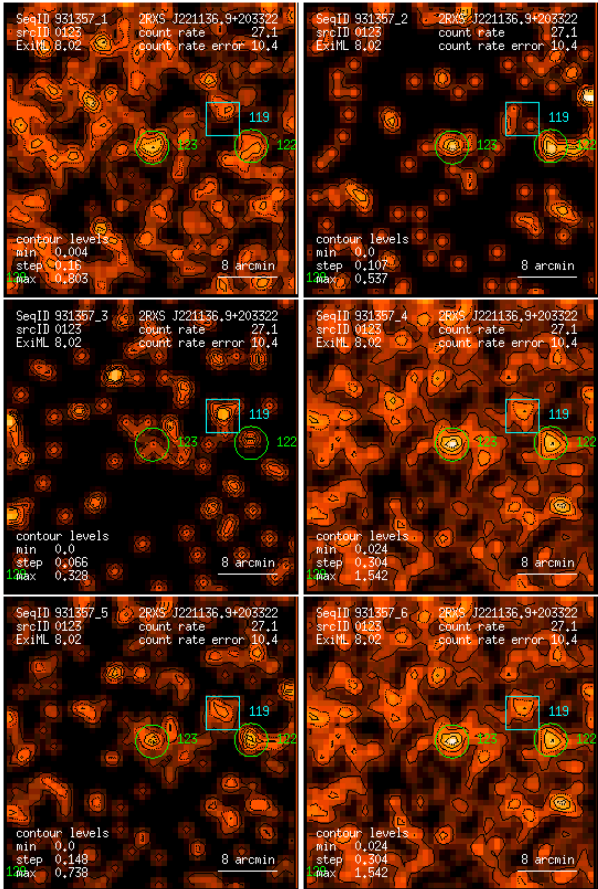
Figure 123: RASS 931357: detection 0123: band rate images, Gaussian filter: (1) PSPC channels 11 – 41, (2) 52 – 90, (3) 91 – 201, (4) 11 – 235, (5) 52 – 201, (6) 11 – 201. Broad band rates in counts/ks. Band rate contour levels in counts/ks/arcmin 2 .
