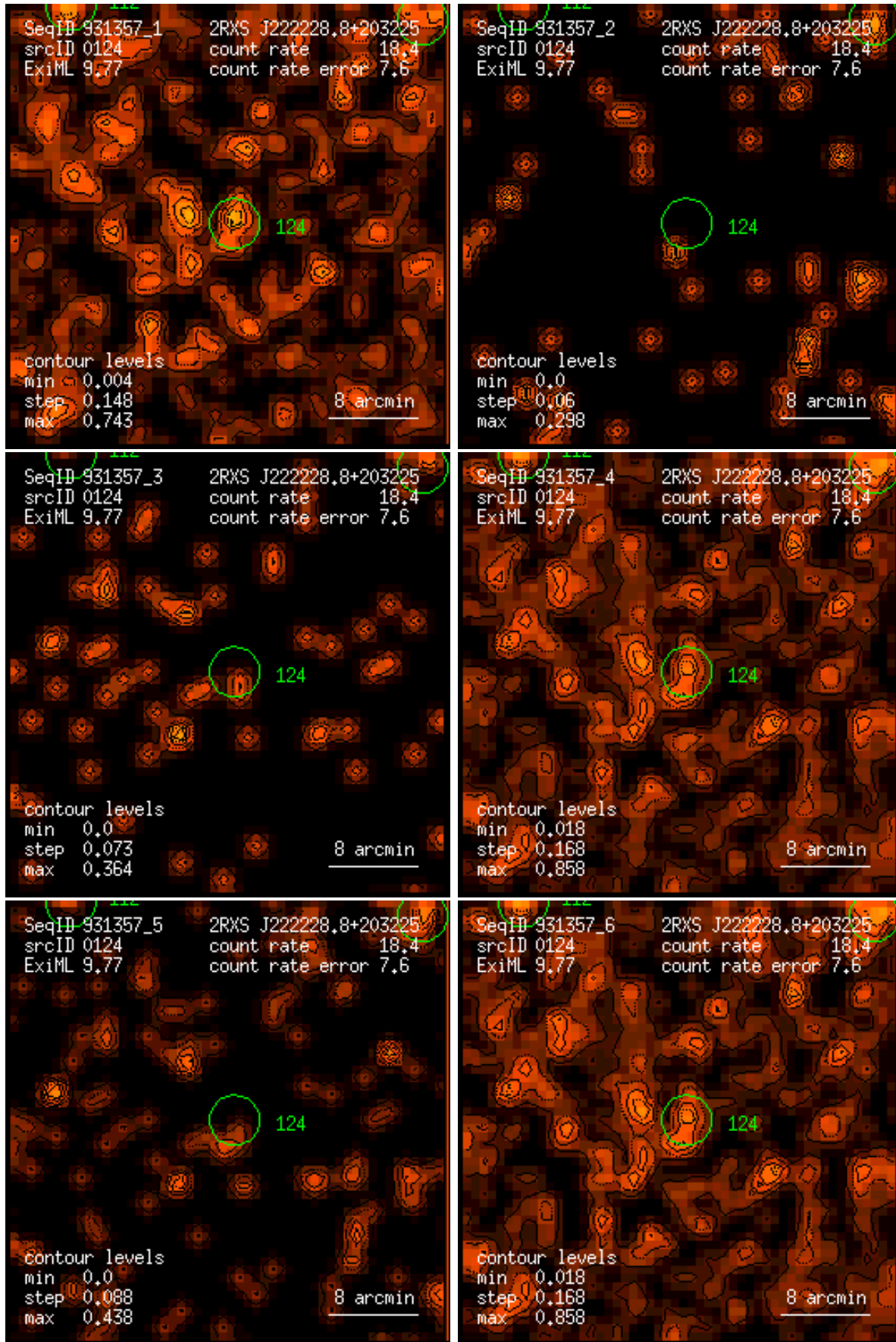
Figure 124: RASS 931357: detection 0124: band rate images, Gaussian filter: (1) PSPC channels 11 – 41, (2) 52 – 90, (3) 91 – 201, (4) 11 – 235, (5) 52 – 201, (6) 11 – 201. Broad band rates in counts/ks. Band rate contour levels in counts/ks/arcmin 2 .
