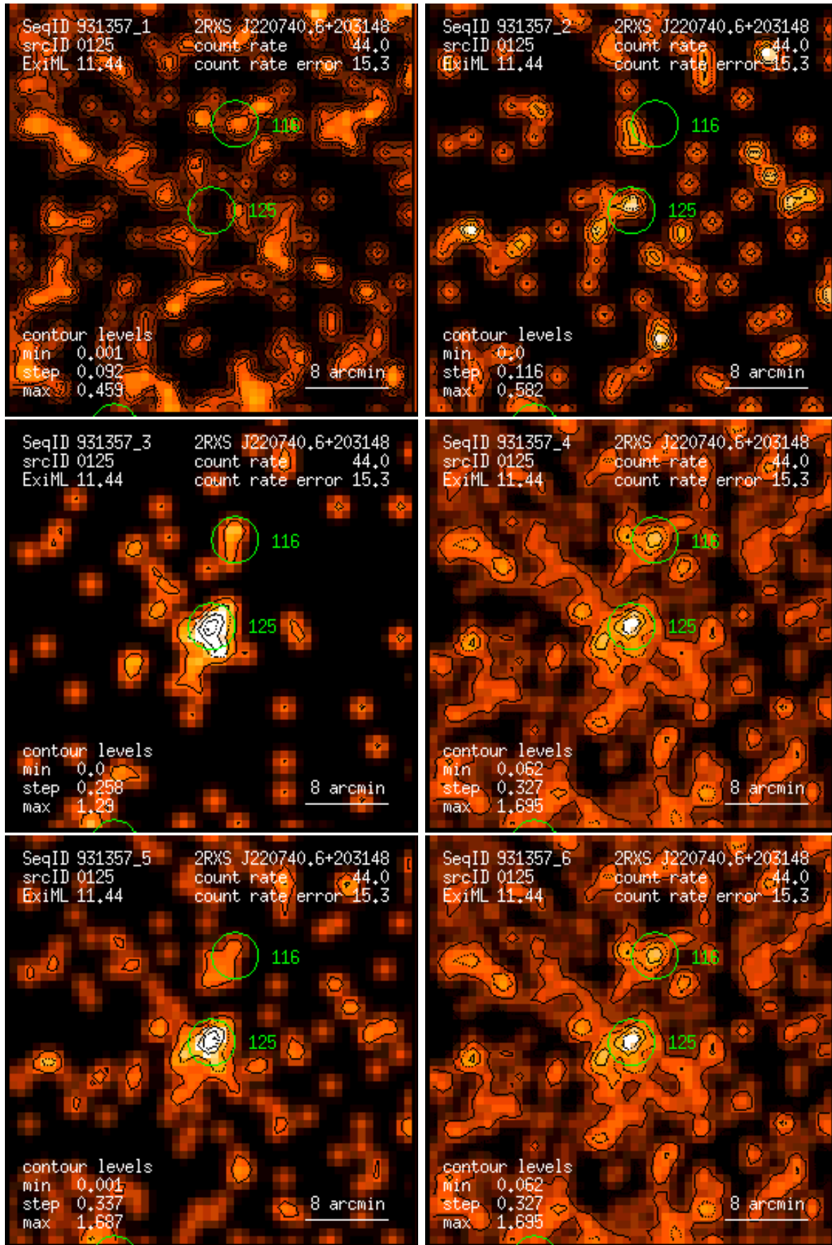
Figure 125: RASS 931357: detection 0125: band rate images, Gaussian filter: (1) PSPC channels 11 – 41, (2) 52 – 90, (3) 91 – 201, (4) 11 – 235, (5) 52 – 201, (6) 11 – 201. Broad band rates in counts/ks. Band rate contour levels in counts/ks/arcmin 2 .
