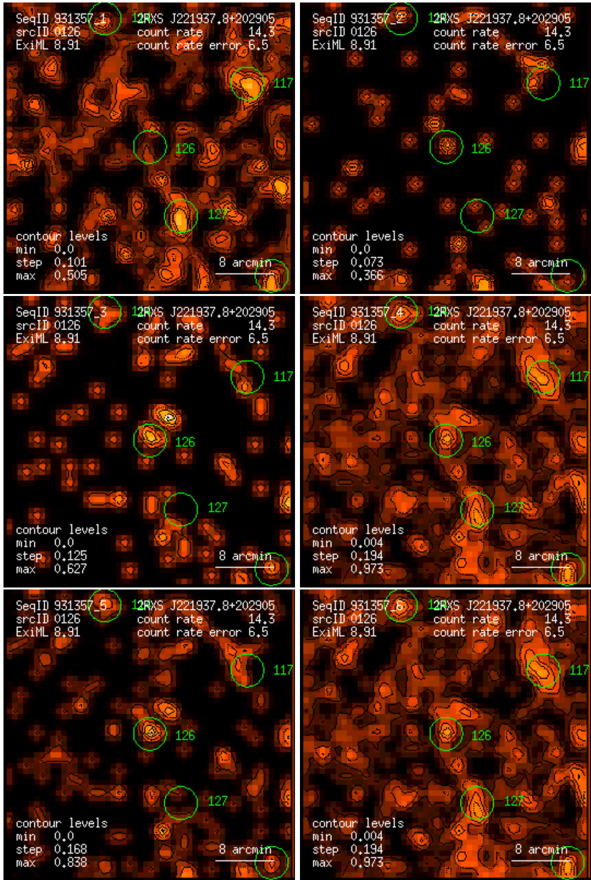
Figure 126: RASS 931357: detection 0126: band rate images, Gaussian filter: (1) PSPC channels 11 – 41, (2) 52 – 90, (3) 91 – 201, (4) 11 – 235, (5) 52 – 201, (6) 11 – 201. Broad band rates in counts/ks. Band rate contour levels in counts/ks/arcmin 2 .
