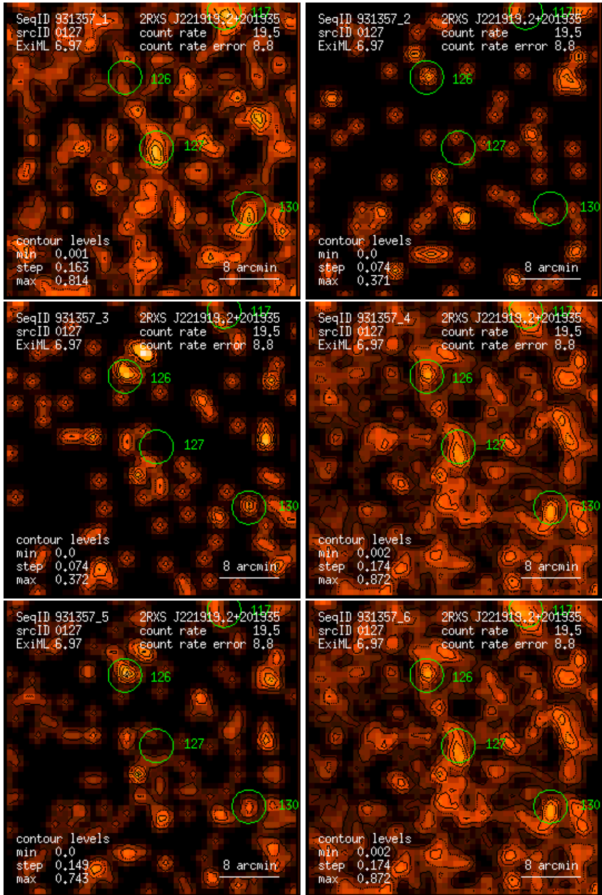
Figure 127: RASS 931357: detection 0127: band rate images, Gaussian filter: (1) PSPC channels 11 – 41, (2) 52 – 90, (3) 91 – 201, (4) 11 – 235, (5) 52 – 201, (6) 11 – 201. Broad band rates in counts/ks. Band rate contour levels in counts/ks/arcmin 2 .
