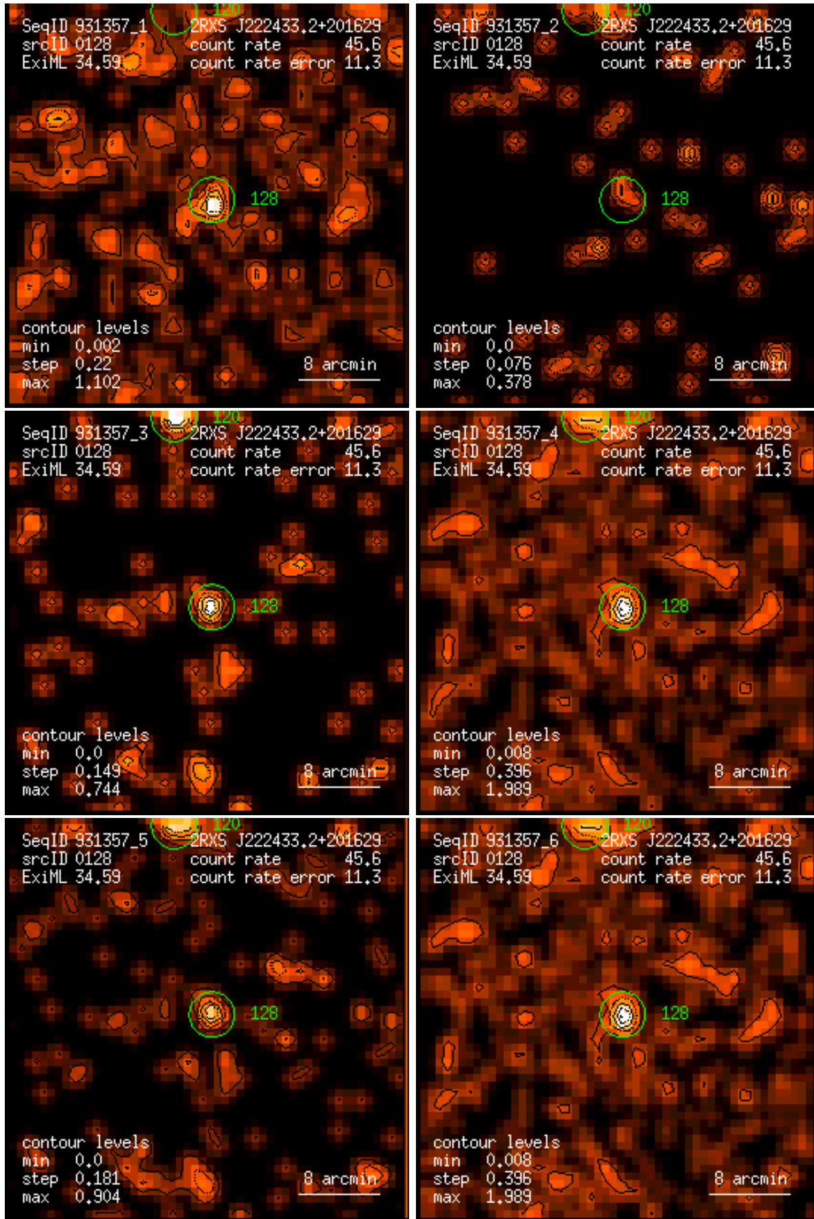
Figure 128: RASS 931357: detection 0128: band rate images, Gaussian filter: (1) PSPC channels 11 – 41, (2) 52 – 90, (3) 91 – 201, (4) 11 – 235, (5) 52 – 201, (6) 11 – 201. Broad band rates in counts/ks. Band rate contour levels in counts/ks/arcmin 2 .
