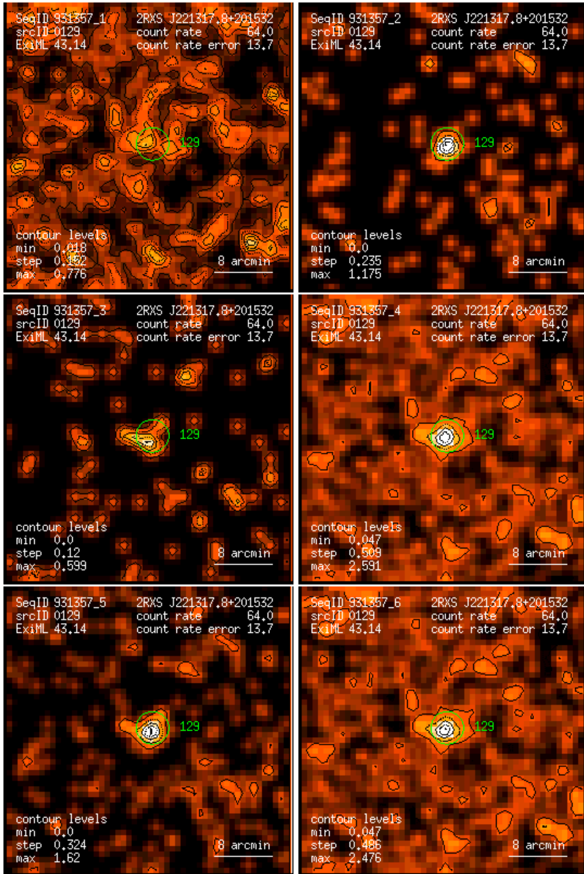
Figure 129: RASS 931357: detection 0129: band rate images, Gaussian filter: (1) PSPC channels 11 – 41, (2) 52 – 90, (3) 91 – 201, (4) 11 – 235, (5) 52 – 201, (6) 11 – 201. Broad band rates in counts/ks. Band rate contour levels in counts/ks/arcmin 2 .
