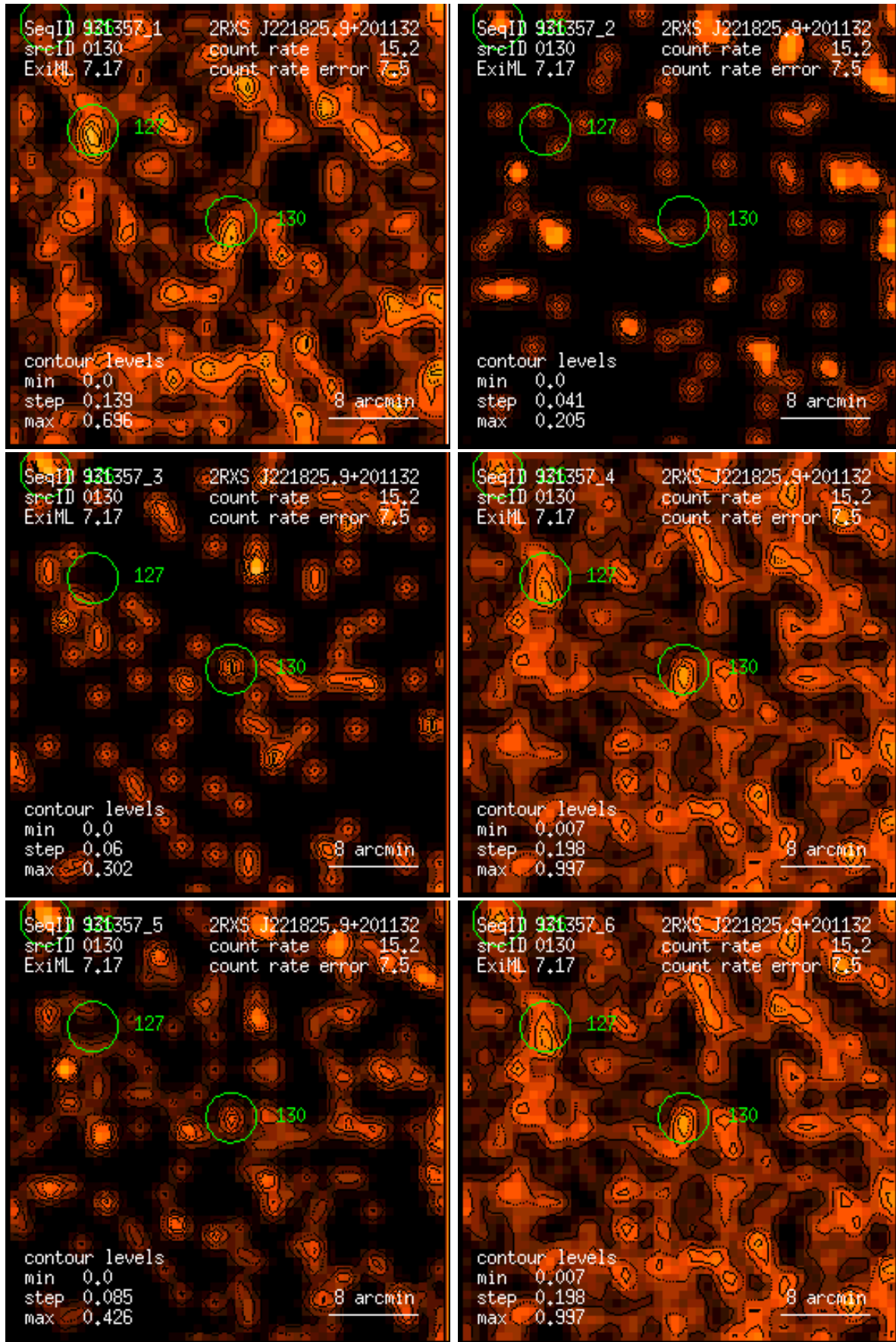
Figure 130: RASS 931357: detection 0130: band rate images, Gaussian filter: (1) PSPC channels 11 – 41, (2) 52 – 90, (3) 91 – 201, (4) 11 – 235, (5) 52 – 201, (6) 11 – 201. Broad band rates in counts/ks. Band rate contour levels in counts/ks/arcmin 2 .
