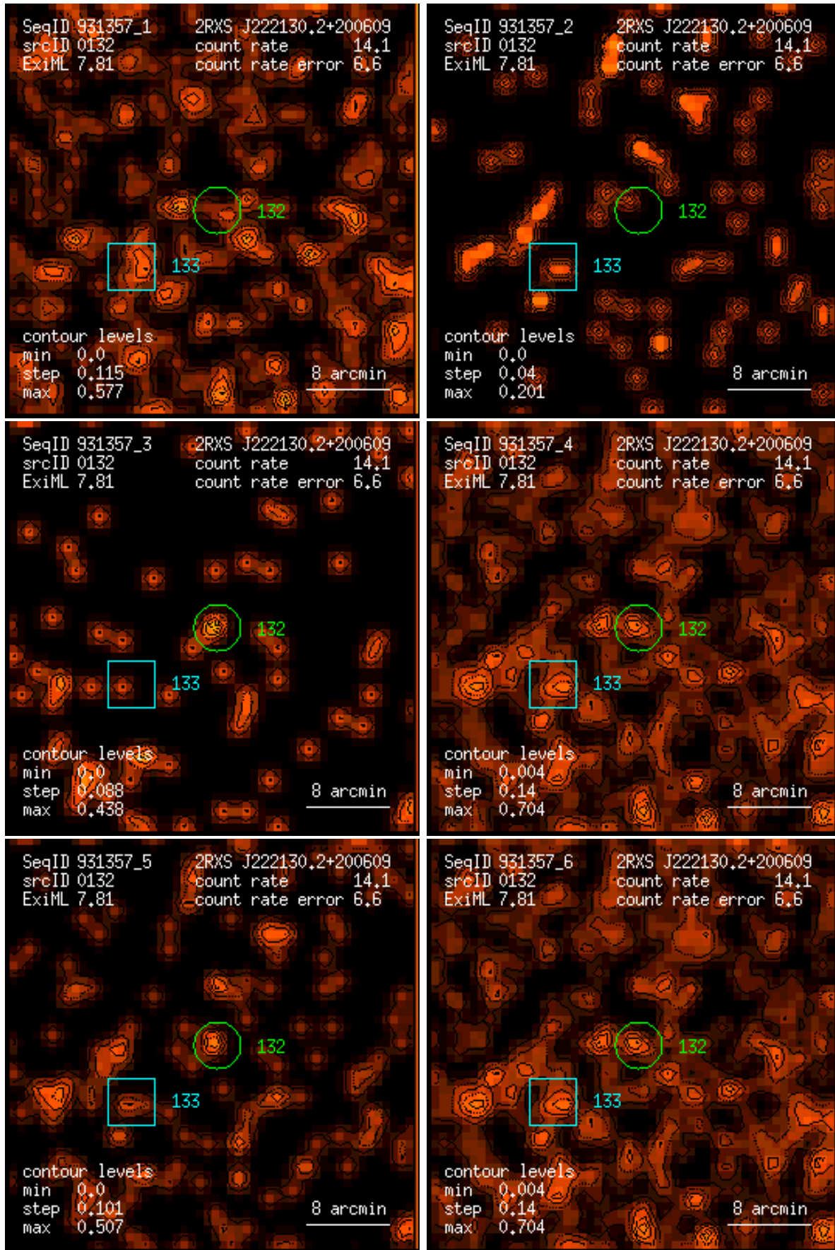
Figure 132: RASS 931357: detection 0132: band rate images, Gaussian filter: (1) PSPC channels 11 – 41, (2) 52 – 90, (3) 91 – 201, (4) 11 – 235, (5) 52 – 201, (6) 11 – 201. Broad band rates in counts/ks. Band rate contour levels in counts/ks/arcmin 2 .
