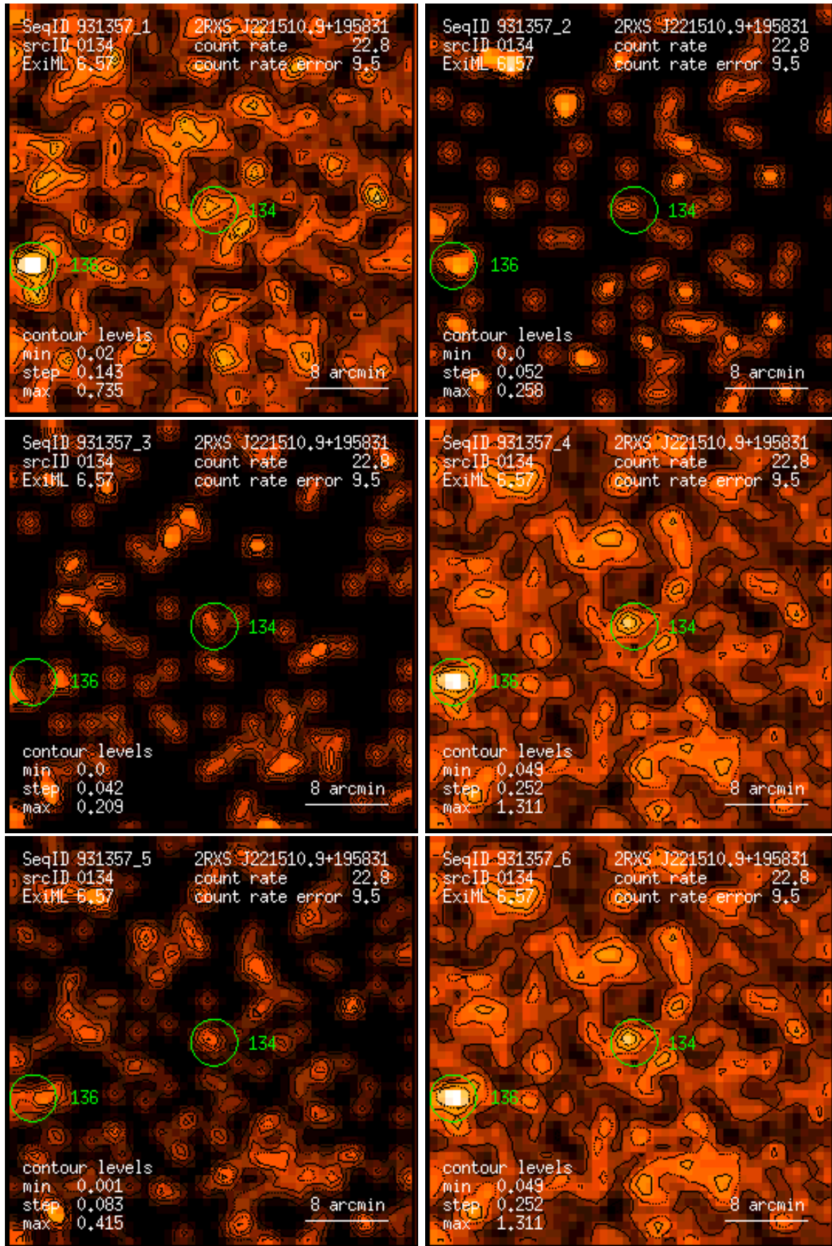
Figure 134: RASS 931357: detection 0134: band rate images, Gaussian filter: (1) PSPC channels 11 – 41, (2) 52 – 90, (3) 91 – 201, (4) 11 – 235, (5) 52 – 201, (6) 11 – 201. Broad band rates in counts/ks. Band rate contour levels in counts/ks/arcmin 2 .
