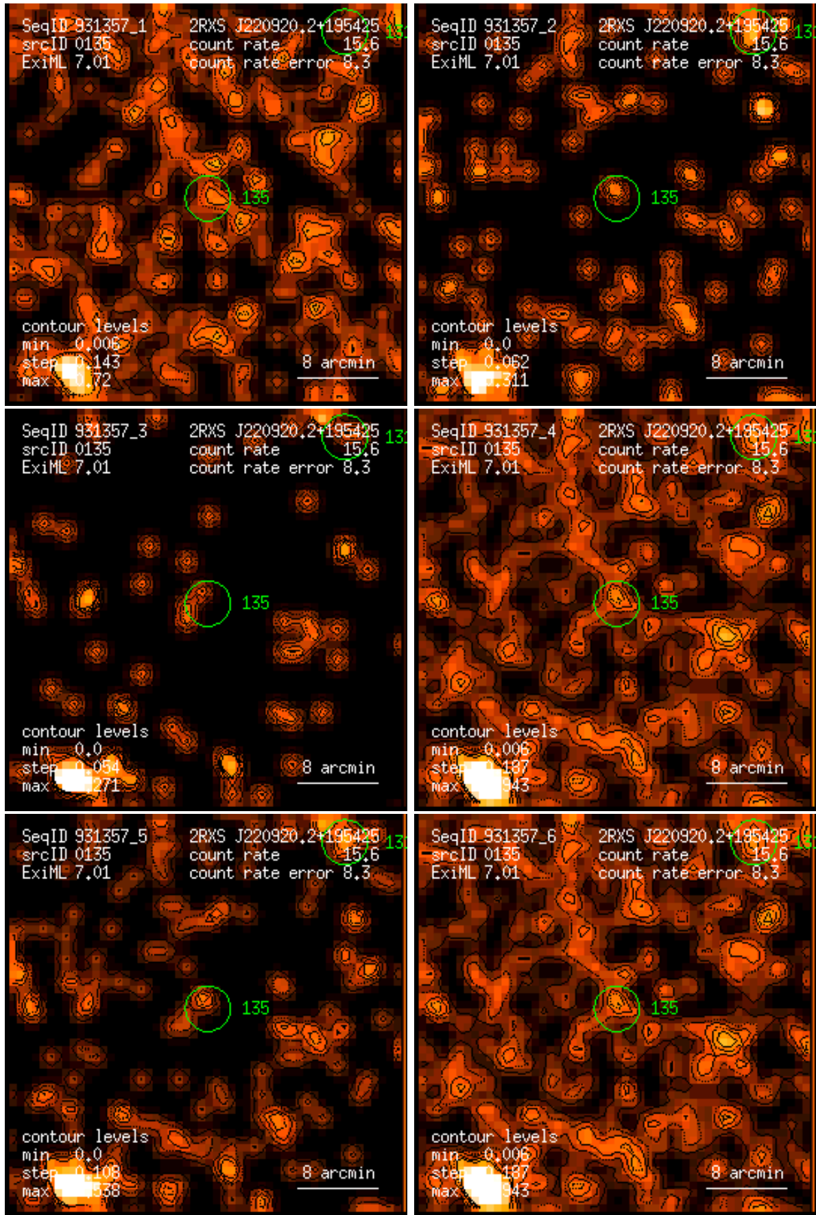
Figure 135: RASS 931357: detection 0135: band rate images, Gaussian filter: (1) PSPC channels 11 – 41, (2) 52 – 90, (3) 91 – 201, (4) 11 – 235, (5) 52 – 201, (6) 11 – 201. Broad band rates in counts/ks. Band rate contour levels in counts/ks/arcmin 2 .
