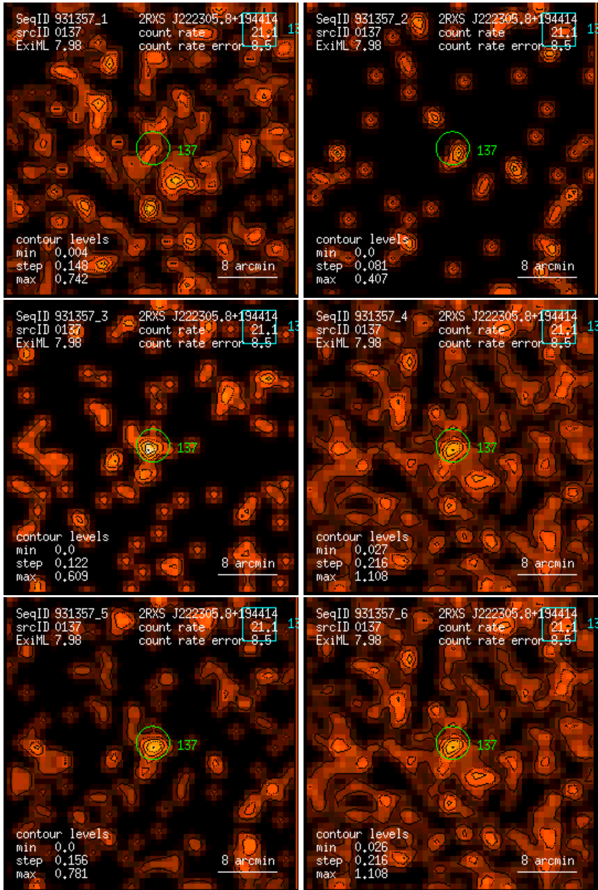
Figure 137: RASS 931357: detection 0137: band rate images, Gaussian filter: (1) PSPC channels 11 – 41, (2) 52 – 90, (3) 91 – 201, (4) 11 – 235, (5) 52 – 201, (6) 11 – 201. Broad band rates in counts/ks. Band rate contour levels in counts/ks/arcmin 2 .
