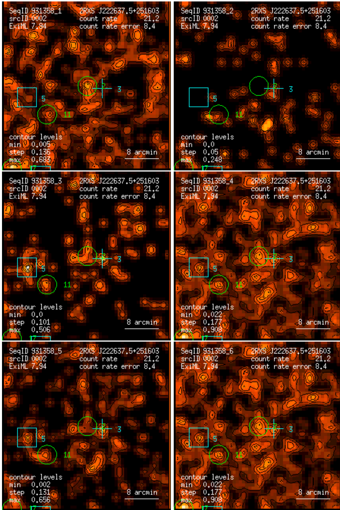
Figure 2: RASS 931358: detection 0002: band rate images, Gaussian filter: (1) PSPC channels 11 – 41, (2) 52 – 90, (3) 91 – 201, (4) 11 – 235, (5) 52 – 201, (6) 11 – 201. Broad band rates in counts/ks. Band rate contour levels in counts/ks/arcmin 2 .
