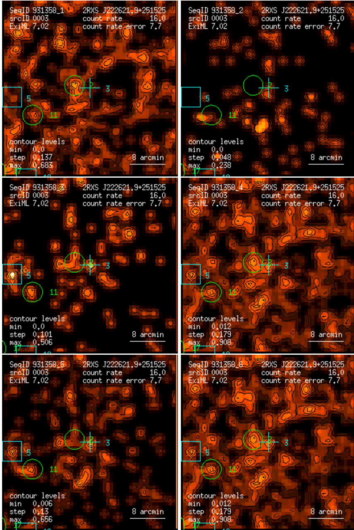
Figure 3: RASS 931358: detection 0003: band rate images, Gaussian filter: (1) PSPC channels 11 – 41, (2) 52 – 90, (3) 91 – 201, (4) 11 – 235, (5) 52 – 201, (6) 11 – 201. Broad band rates in counts/ks. Band rate contour levels in counts/ks/arcmin 2 .
