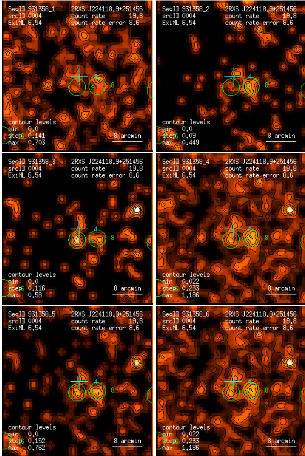
Figure 4: RASS 931358: detection 0004: band rate images, Gaussian filter: (1) PSPC channels 11 – 41, (2) 52 – 90, (3) 91 – 201, (4) 11 – 235, (5) 52 – 201, (6) 11 – 201. Broad band rates in counts/ks. Band rate contour levels in counts/ks/arcmin 2 .
