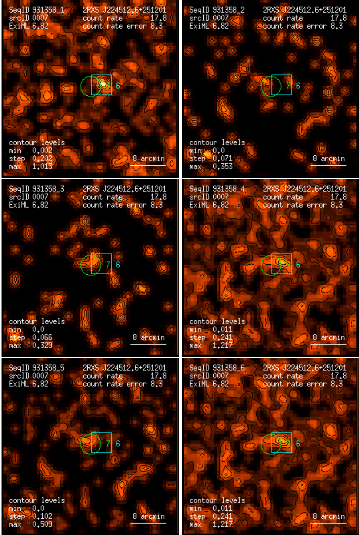
Figure 7: RASS 931358: detection 0007: band rate images, Gaussian filter: (1) PSPC channels 11 – 41, (2) 52 – 90, (3) 91 – 201, (4) 11 – 235, (5) 52 – 201, (6) 11 – 201. Broad band rates in counts/ks. Band rate contour levels in counts/ks/arcmin 2 .
