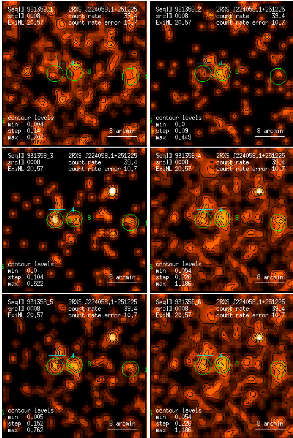
Figure 8: RASS 931358: detection 0008: band rate images, Gaussian filter: (1) PSPC channels 11 – 41, (2) 52 – 90, (3) 91 – 201, (4) 11 – 235, (5) 52 – 201, (6) 11 – 201. Broad band rates in counts/ks. Band rate contour levels in counts/ks/arcmin 2 .
