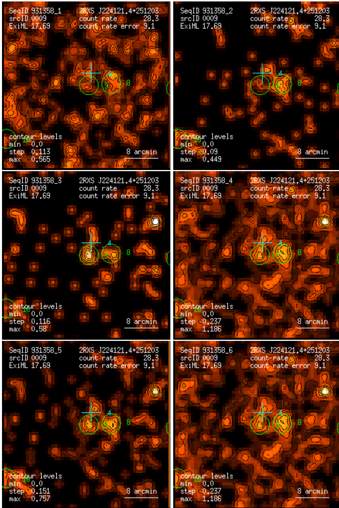
Figure 9: RASS 931358: detection 0009: band rate images, Gaussian filter: (1) PSPC channels 11 – 41, (2) 52 – 90, (3) 91 – 201, (4) 11 – 235, (5) 52 – 201, (6) 11 – 201. Broad band rates in counts/ks. Band rate contour levels in counts/ks/arcmin 2 .
