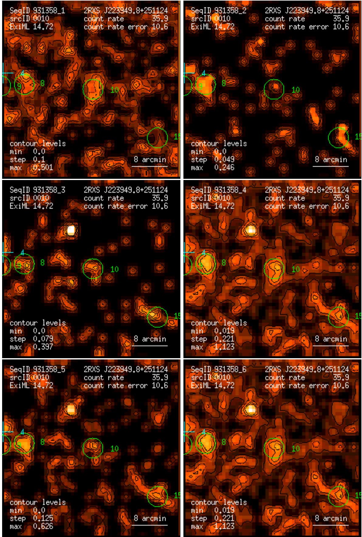
Figure 10: RASS 931358: detection 0010: band rate images, Gaussian filter: (1) PSPC channels 11 – 41, (2) 52 – 90, (3) 91 – 201, (4) 11 – 235, (5) 52 – 201, (6) 11 – 201. Broad band rates in counts/ks. Band rate contour levels in counts/ks/arcmin 2 .
