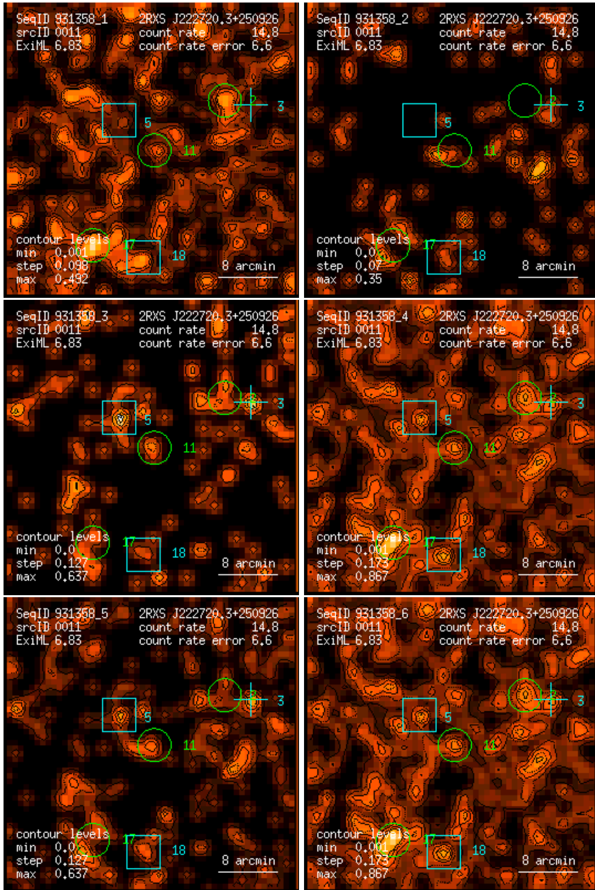
Figure 11: RASS 931358: detection 0011: band rate images, Gaussian filter: (1) PSPC channels 11 – 41, (2) 52 – 90, (3) 91 – 201, (4) 11 – 235, (5) 52 – 201, (6) 11 – 201. Broad band rates in counts/ks. Band rate contour levels in counts/ks/arcmin 2 .
