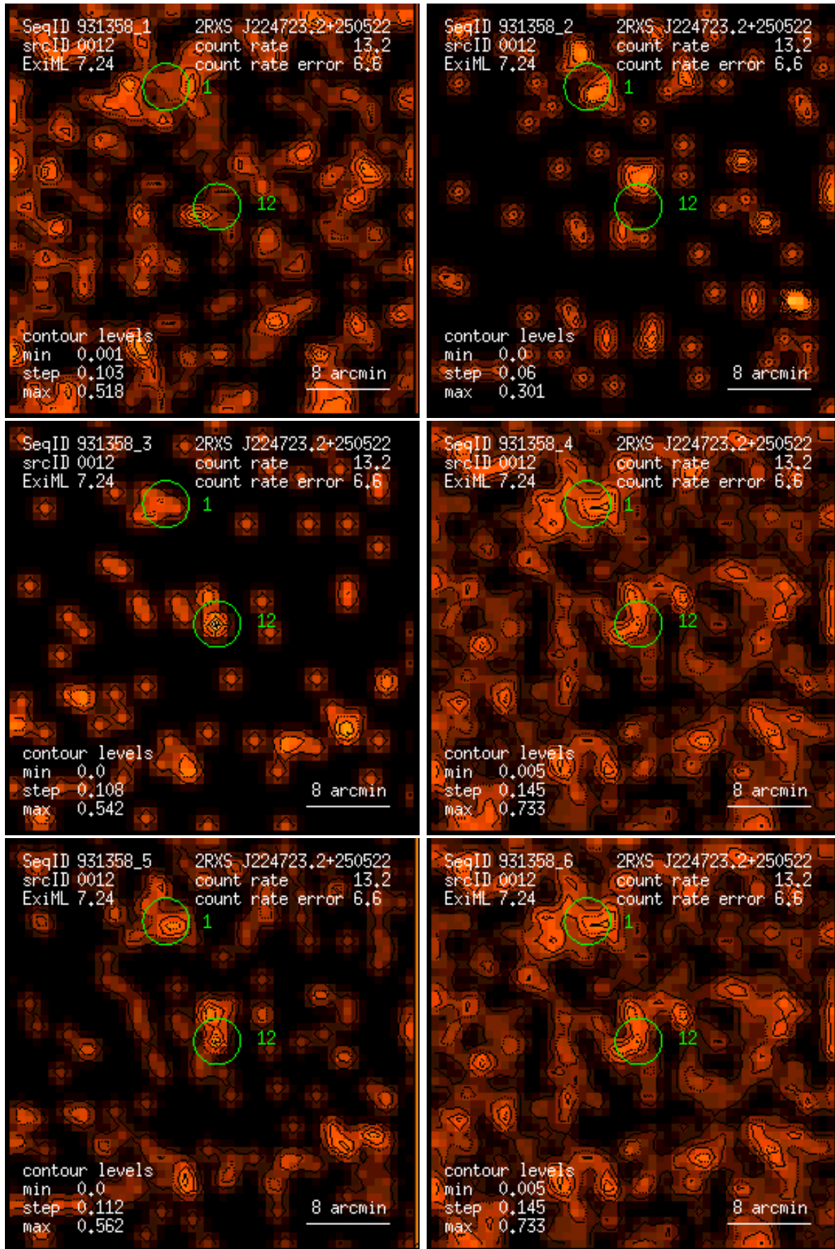
Figure 12: RASS 931358: detection 0012: band rate images, Gaussian filter: (1) PSPC channels 11 – 41, (2) 52 – 90, (3) 91 – 201, (4) 11 – 235, (5) 52 – 201, (6) 11 – 201. Broad band rates in counts/ks. Band rate contour levels in counts/ks/arcmin 2 .
