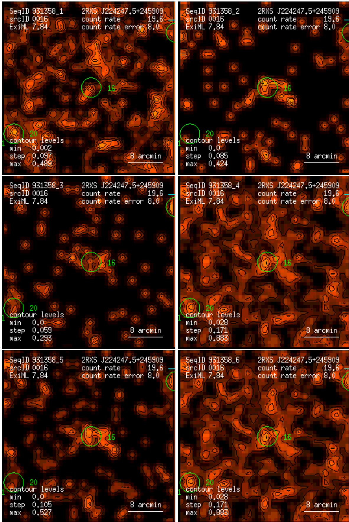
Figure 16: RASS 931358: detection 0016: band rate images, Gaussian filter: (1) PSPC channels 11 – 41, (2) 52 – 90, (3) 91 – 201, (4) 11 – 235, (5) 52 – 201, (6) 11 – 201. Broad band rates in counts/ks. Band rate contour levels in counts/ks/arcmin 2 .
