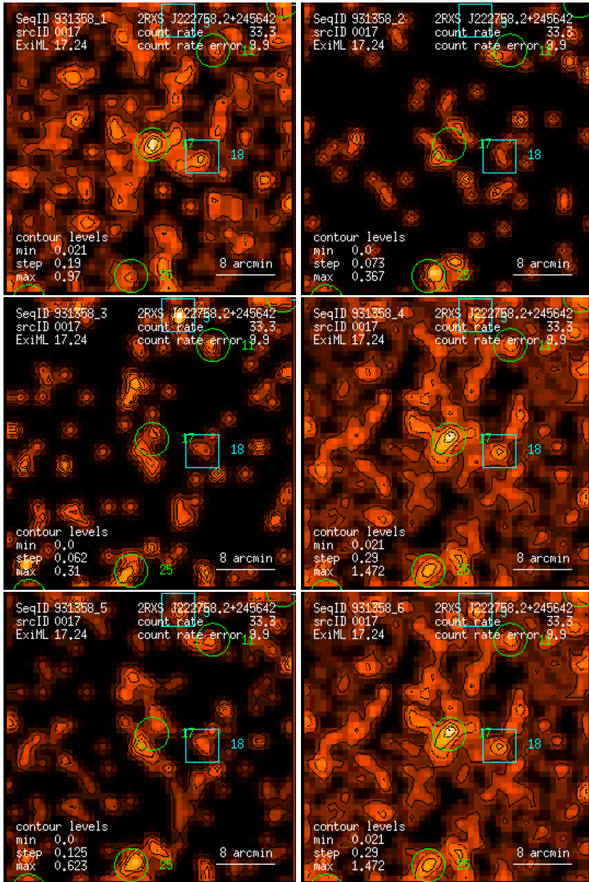
Figure 17: RASS 931358: detection 0017: band rate images, Gaussian filter: (1) PSPC channels 11 – 41, (2) 52 – 90, (3) 91 – 201, (4) 11 – 235, (5) 52 – 201, (6) 11 – 201. Broad band rates in counts/ks. Band rate contour levels in counts/ks/arcmin 2 .
