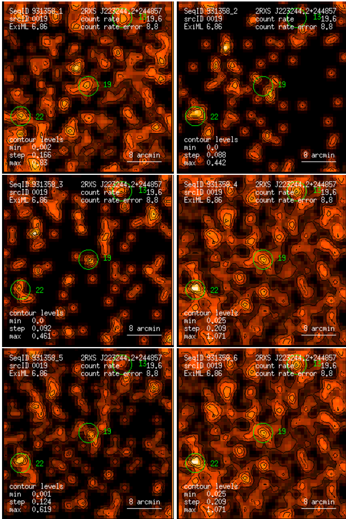
Figure 19: RASS 931358: detection 0019: band rate images, Gaussian filter: (1) PSPC channels 11 – 41, (2) 52 – 90, (3) 91 – 201, (4) 11 – 235, (5) 52 – 201, (6) 11 – 201. Broad band rates in counts/ks. Band rate contour levels in counts/ks/arcmin 2 .
