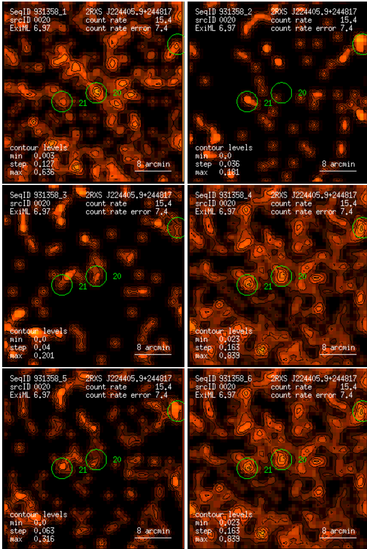
Figure 20: RASS 931358: detection 0020: band rate images, Gaussian filter: (1) PSPC channels 11 – 41, (2) 52 – 90, (3) 91 – 201, (4) 11 – 235, (5) 52 – 201, (6) 11 – 201. Broad band rates in counts/ks. Band rate contour levels in counts/ks/arcmin 2 .
