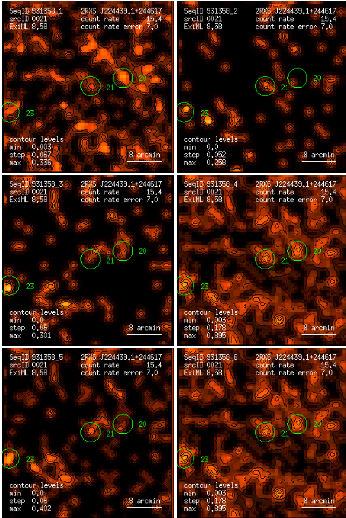
Figure 21: RASS 931358: detection 0021: band rate images, Gaussian filter: (1) PSPC channels 11 – 41, (2) 52 – 90, (3) 91 – 201, (4) 11 – 235, (5) 52 – 201, (6) 11 – 201. Broad band rates in counts/ks. Band rate contour levels in counts/ks/arcmin 2 .
