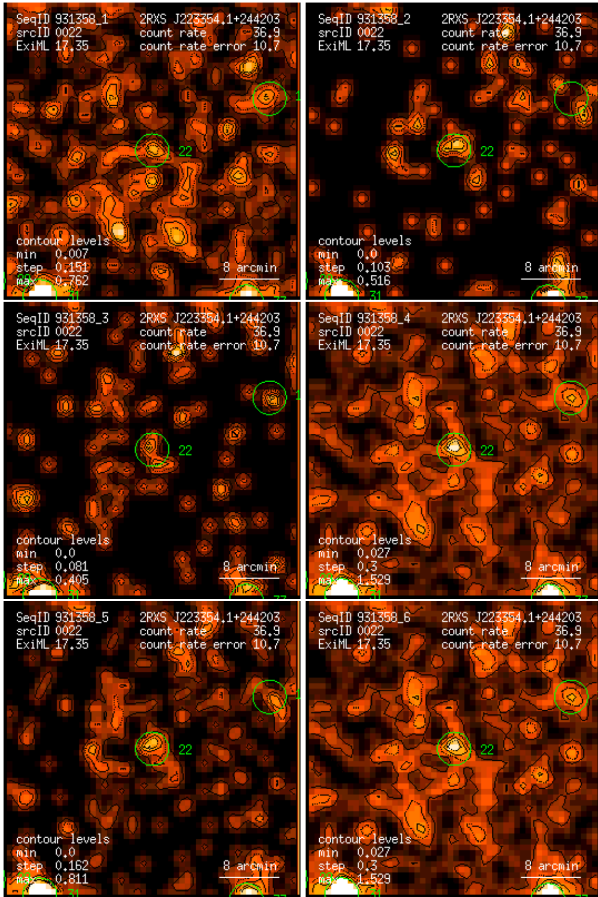
Figure 22: RASS 931358: detection 0022: band rate images, Gaussian filter: (1) PSPC channels 11 – 41, (2) 52 – 90, (3) 91 – 201, (4) 11 – 235, (5) 52 – 201, (6) 11 – 201. Broad band rates in counts/ks. Band rate contour levels in counts/ks/arcmin 2 .
