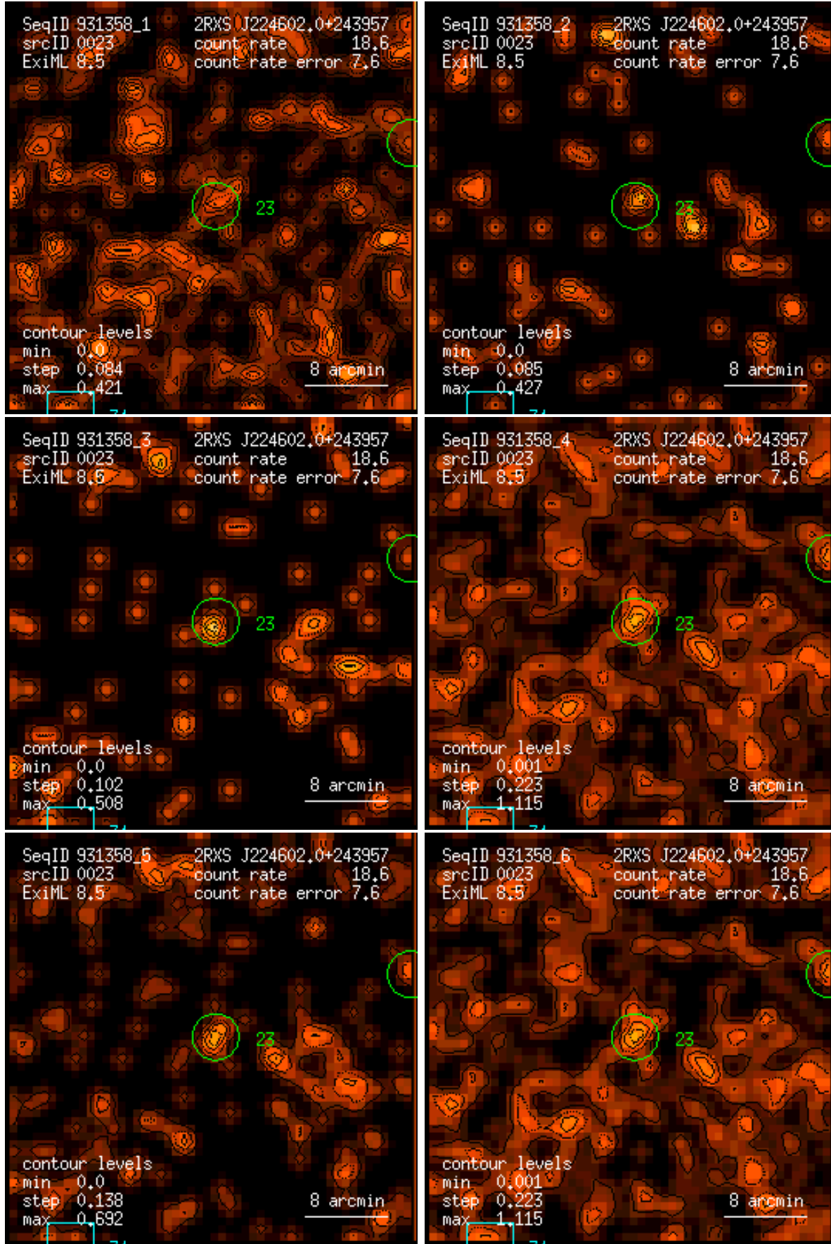
Figure 23: RASS 931358: detection 0023: band rate images, Gaussian filter: (1) PSPC channels 11 – 41, (2) 52 – 90, (3) 91 – 201, (4) 11 – 235, (5) 52 – 201, (6) 11 – 201. Broad band rates in counts/ks. Band rate contour levels in counts/ks/arcmin 2 .
