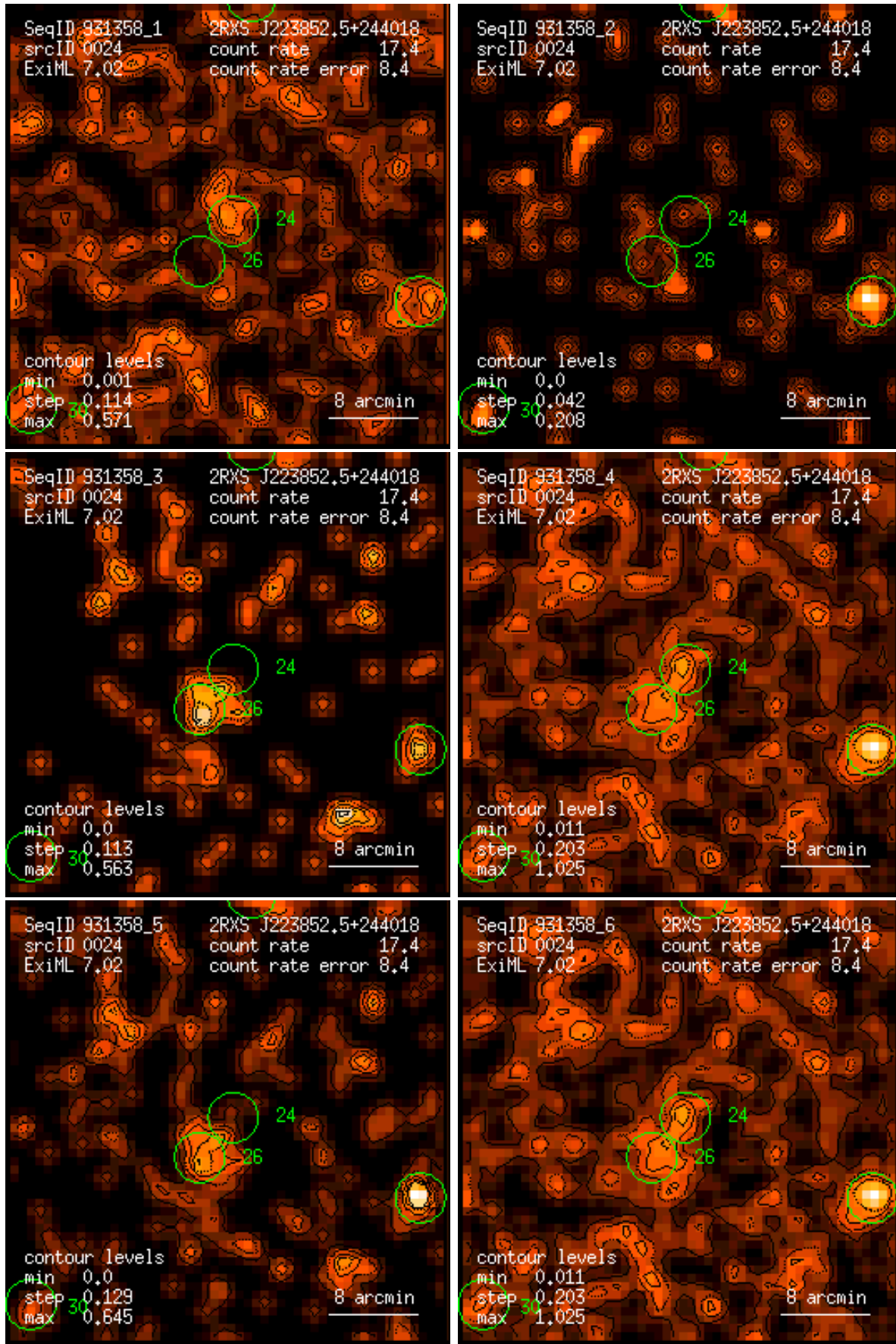
Figure 24: RASS 931358: detection 0024: band rate images, Gaussian filter: (1) PSPC channels 11 – 41, (2) 52 – 90, (3) 91 – 201, (4) 11 – 235, (5) 52 – 201, (6) 11 – 201. Broad band rates in counts/ks. Band rate contour levels in counts/ks/arcmin 2 .
