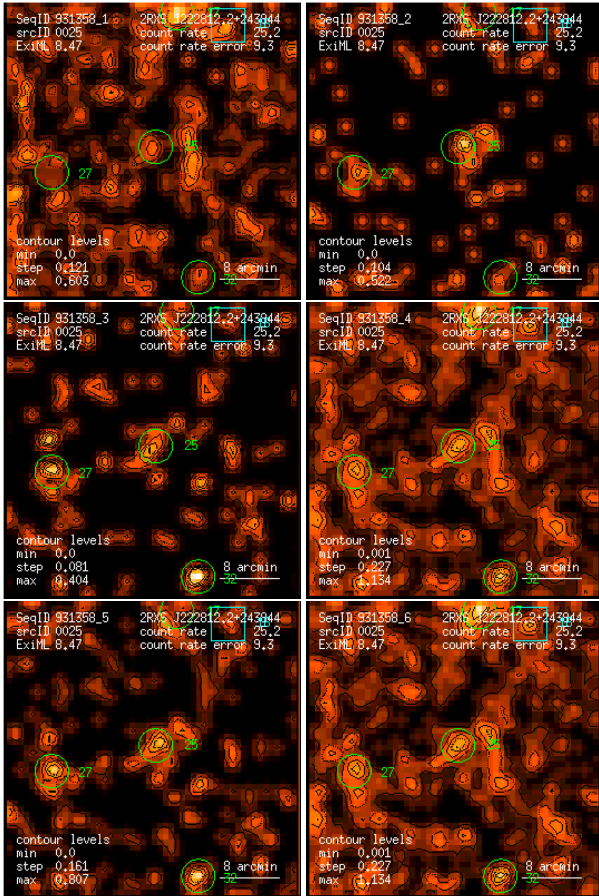
Figure 25: RASS 931358: detection 0025: band rate images, Gaussian filter: (1) PSPC channels 11 – 41, (2) 52 – 90, (3) 91 – 201, (4) 11 – 235, (5) 52 – 201, (6) 11 – 201. Broad band rates in counts/ks. Band rate contour levels in counts/ks/arcmin 2 .
